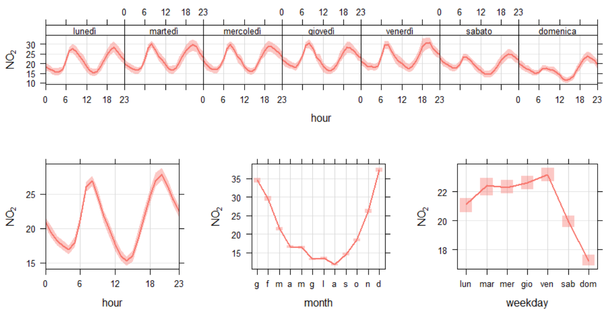
mean and 95% confidence interval in mean Fig. 4.16: NO 2 – Andamenti (µg/m 3 ).
