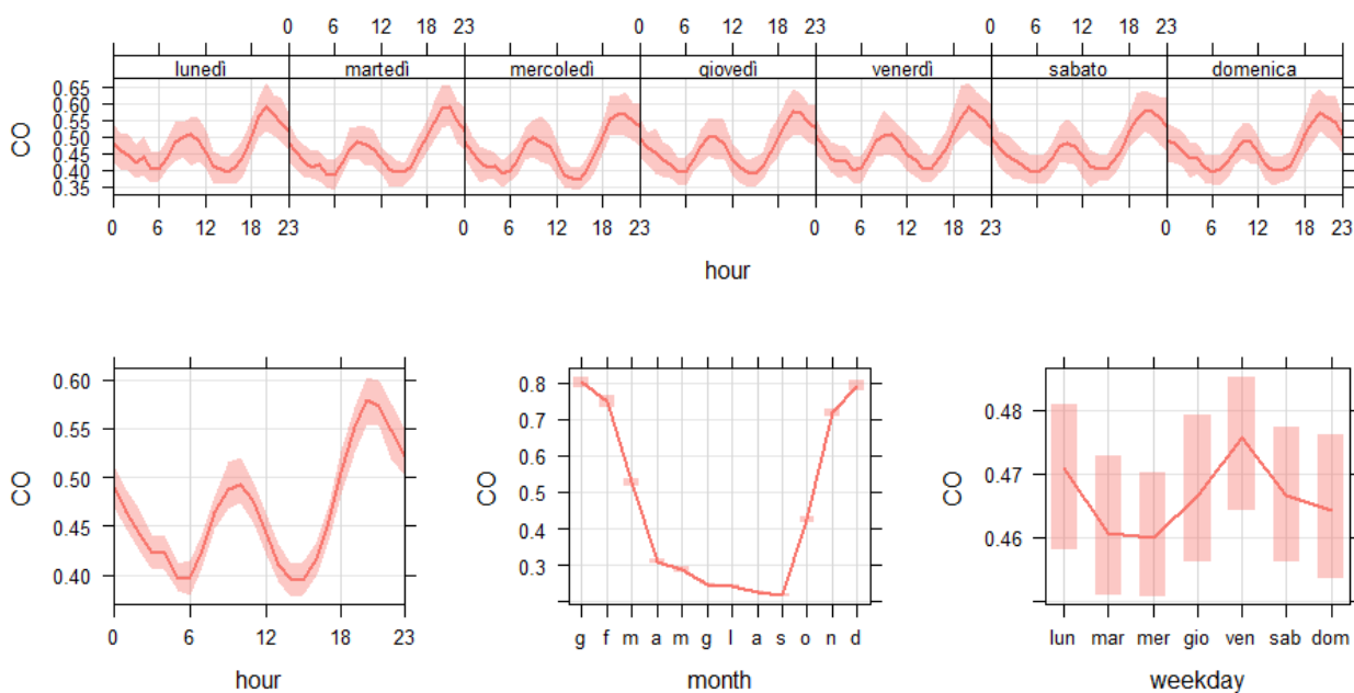
mean and 95% confidence interval in mean Fig. 4.3: CO – Andamenti ( \text{mg/m}^3 ).
