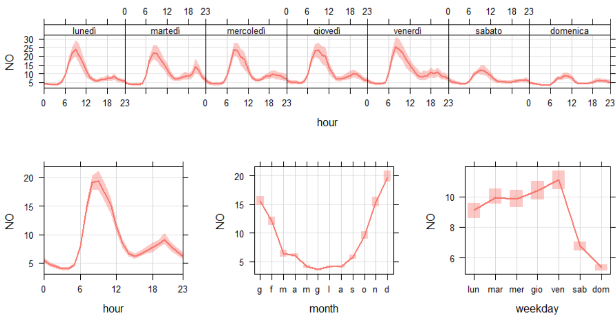
mean and 95% confidence interval in mean Fig. 4.17: NO – Andamenti ( \mu\text{g}/\text{m}^3 ).
